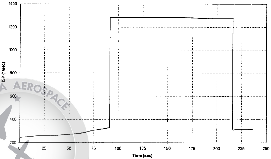
NASAE3CTH2O2/JPB4 Specific Impulse vs Time
