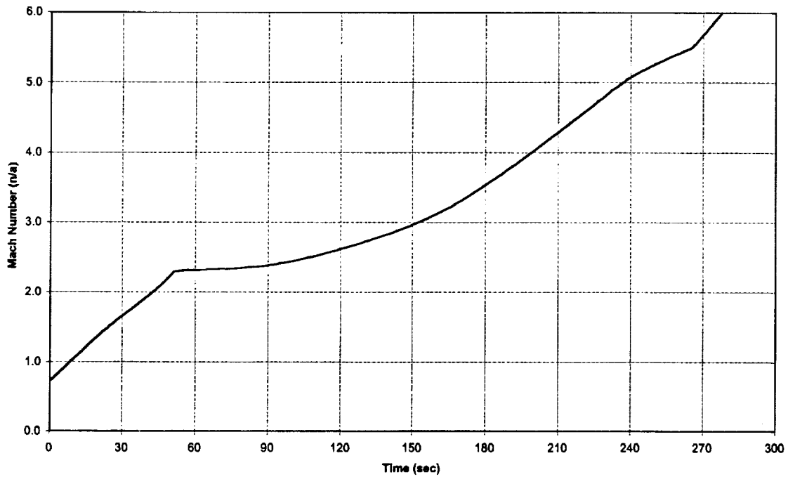
NASAE3GTH2O2/JPA Mach vs Time
