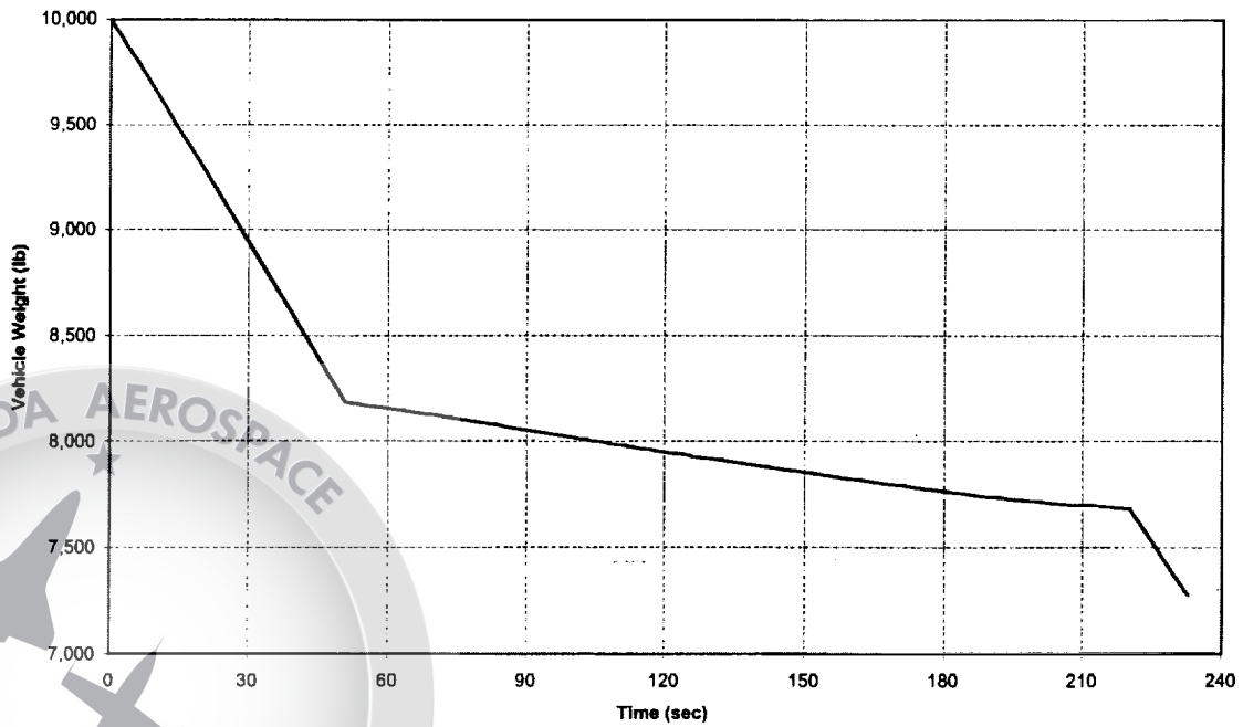
NASAE3GTLOX/JPA Weight vs Time
