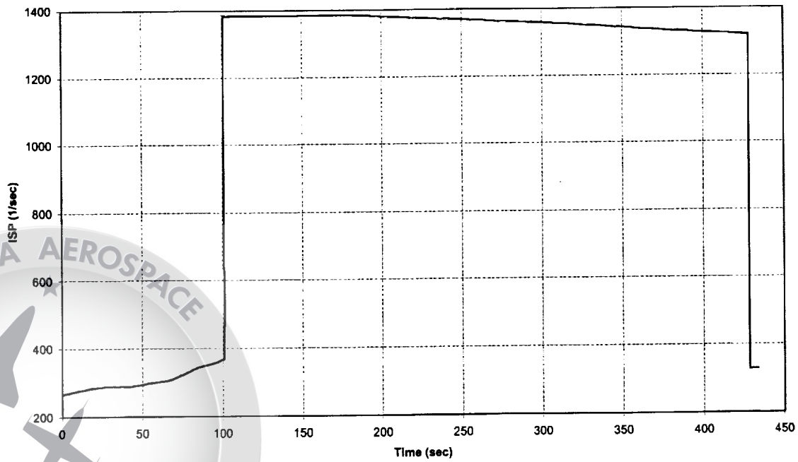
NASAE3CTLOX/ProC1 Specific Impulse vs Time
