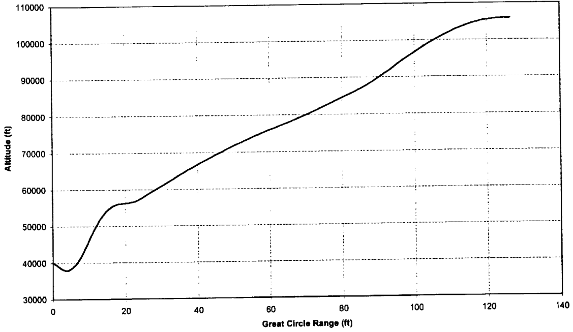
NASAE3GTLOX/PRA Altitude vs Great Circle Range
