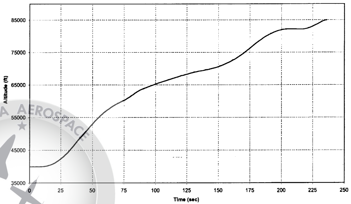
NASAE3CTH2O2/JPB4 Altitude vs Time
