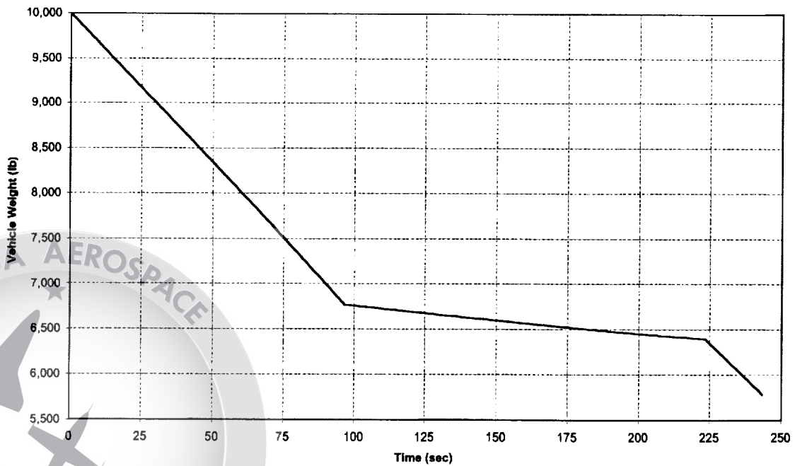
NASAE3CTLOX/ProB4 Weight vs Time
