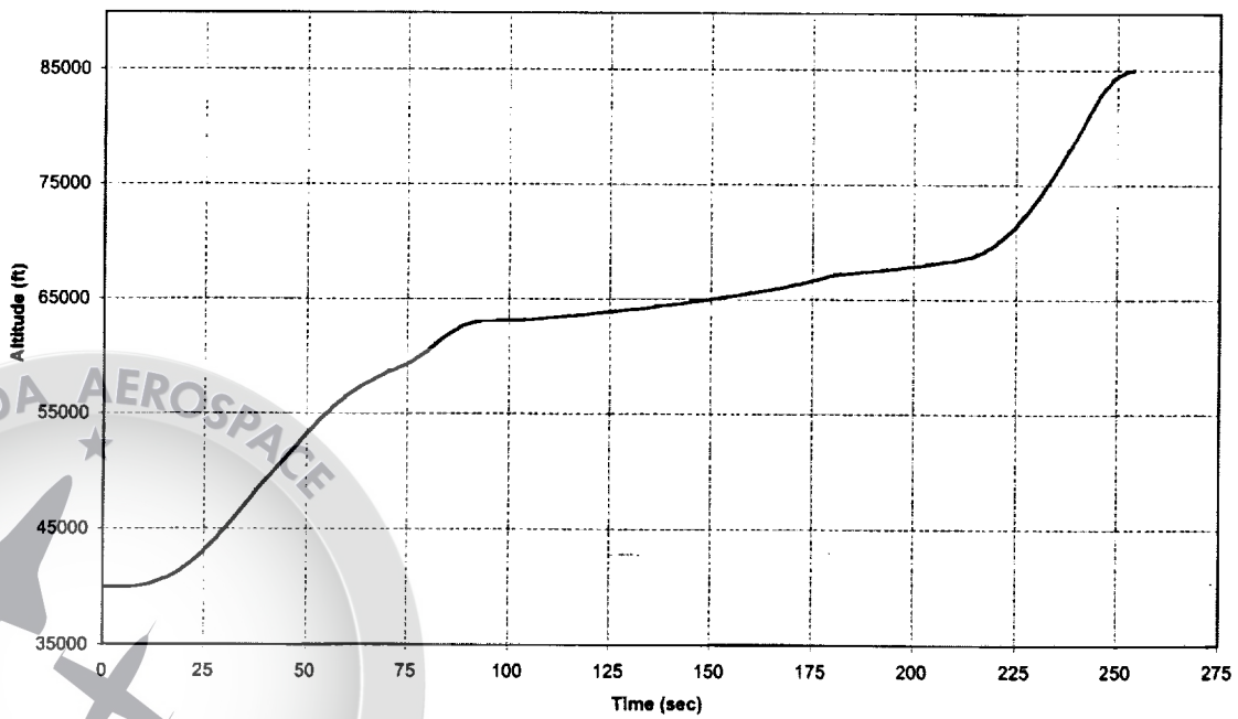
NASAE3CTH2O2/JPC1 Altitude vs Time
