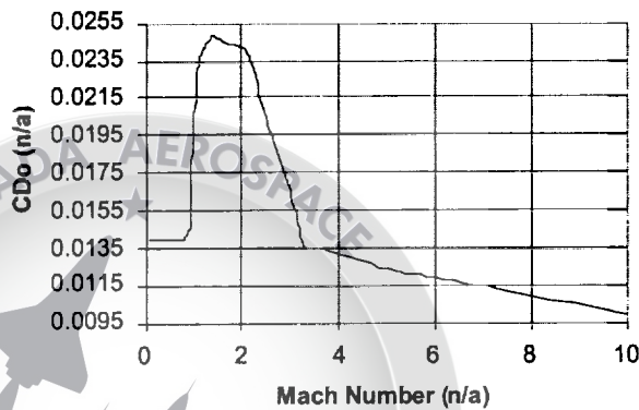
Figure 4.1: C_{Do} vs Mach Number
