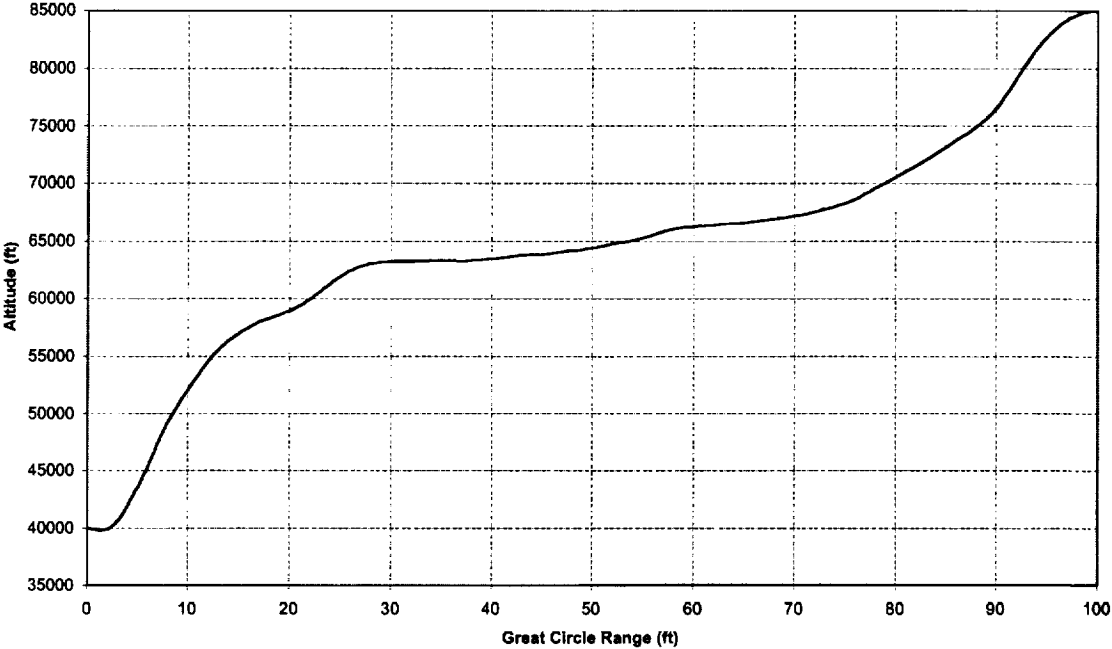
NASAE3CTLOX/ProB4 Altitude vs Great Circle Range
