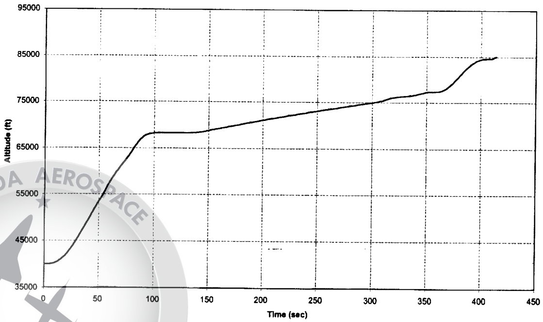
NASAE3CTLOX/JPC1 Altitude vs Time
