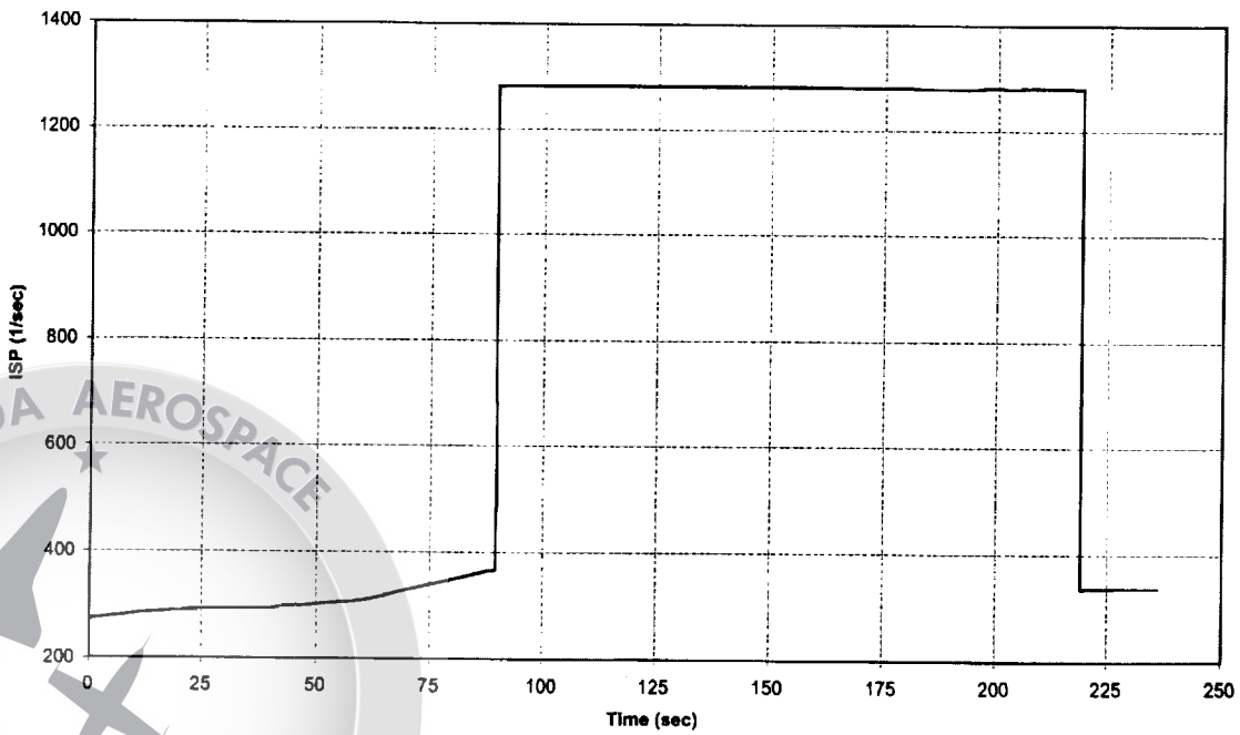
NASAE3CTLOXJPB4 Specific Impulse vs Time
