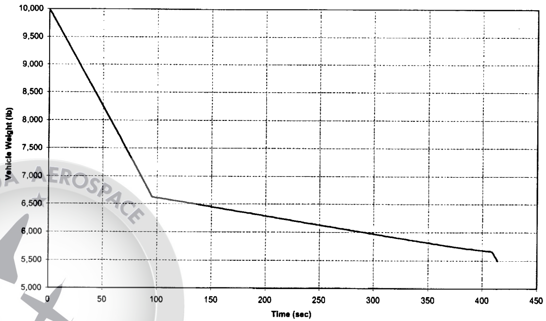
NASAE3CTLOX/JPC1 Weight vs Time
