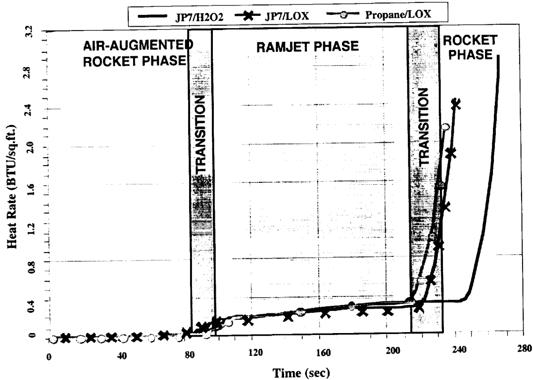
Figure 4.9: Comparison of Heat Rates Over Time
