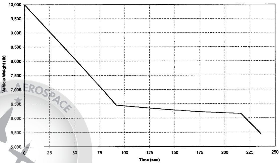
NASAE3CTH2O2/JPB4 Weight vs Time
