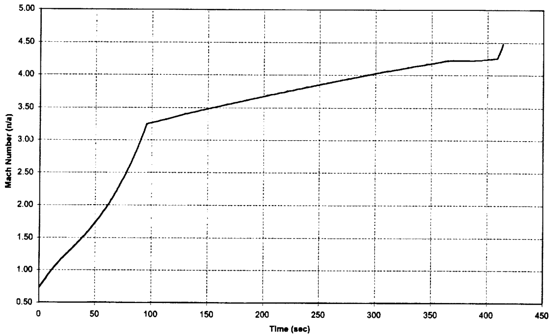
NASAE3CTLOX/JPC1 Mach vs Time
