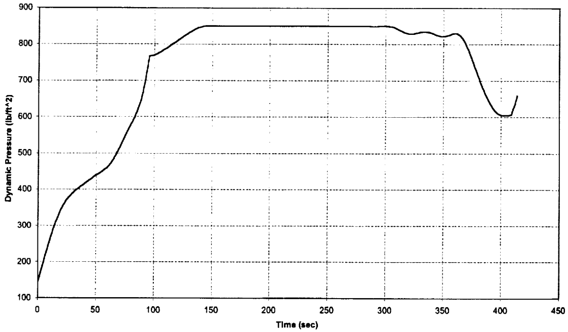
NASAE3CTLOX/JPC1 Dynamic Pressure vs Time
