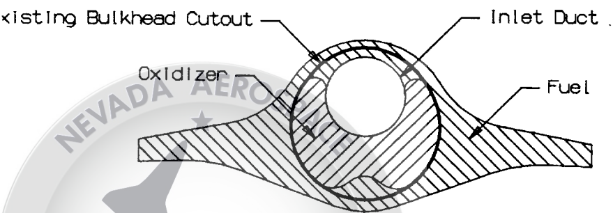
Section B-B Rotated CW 90 deg F.S. 272.5 View Looking Aft
