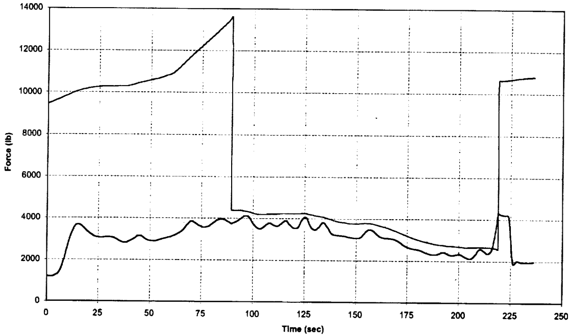
NASAE3CTLOX/JPB4 Thrust & Drag vs Time
