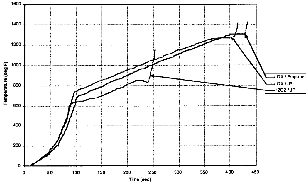
Figure 4.5: Final Trajectory Propellant Nose Temperature Profiles
