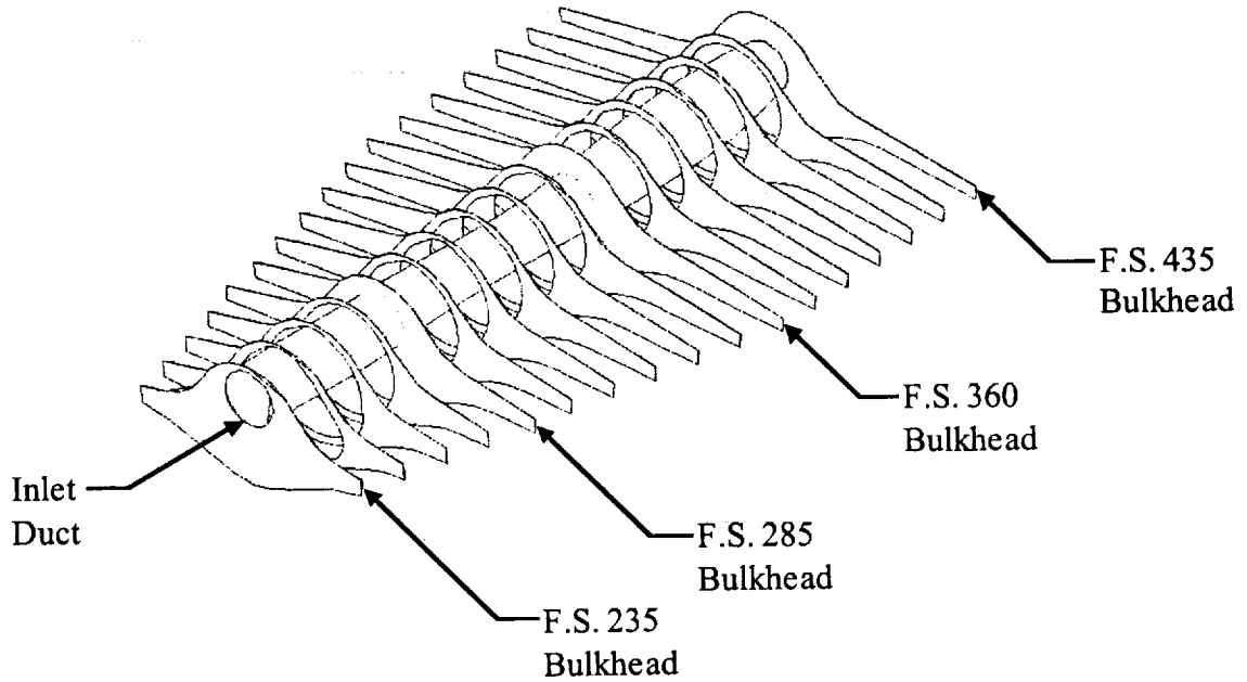
Figure 5.2: D-21 Fuel Tank Bulkheads and Frames
