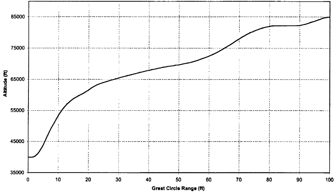
NASAE3CTH2O2/JPB4 Altitude vs Great Circle Range
