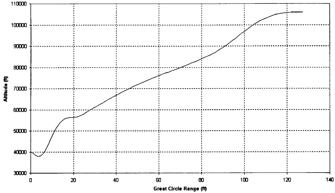
NASAE3GTLOXJPA Altitude vs Great Circle Range
