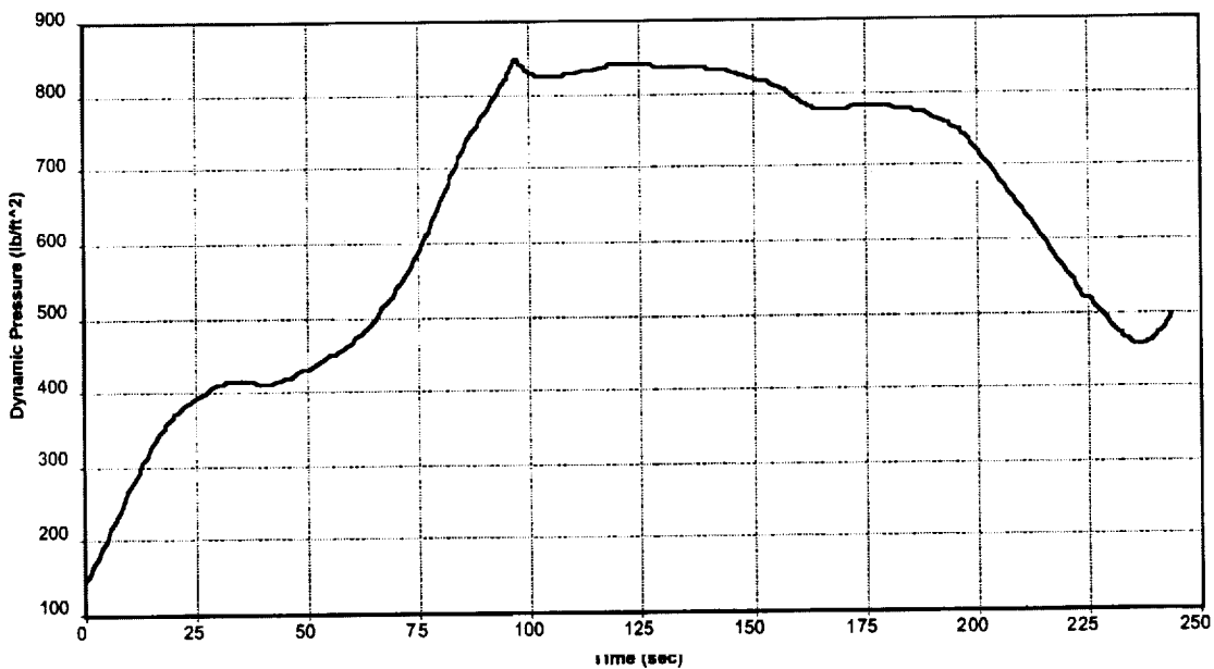
Figure 4.10: NASA E3CTLOX/ProB4 Dynamic Pressure vs Time
