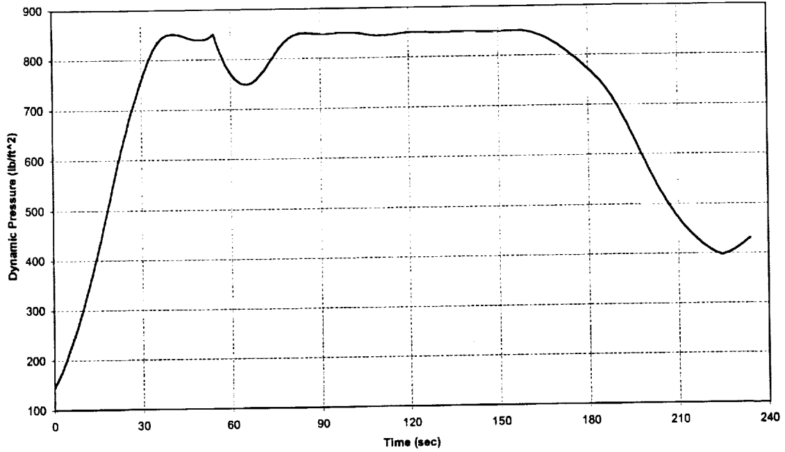
NASAE3GTLOX/PRA Dynamic Pressure vs Time
