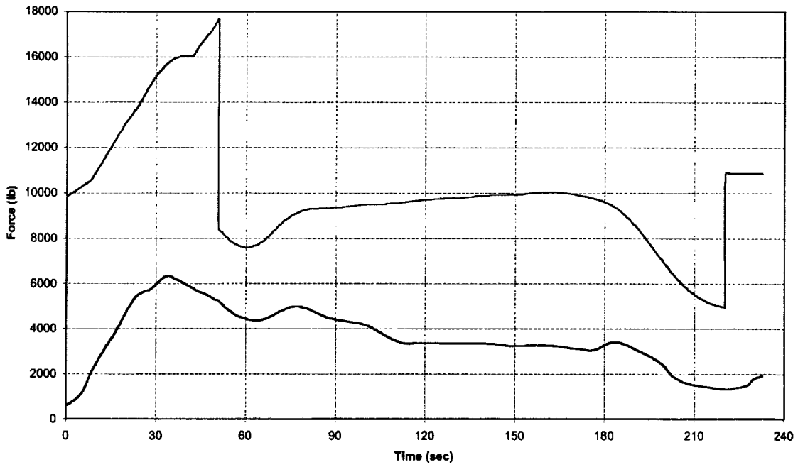
NASAE3GTLOX/JPA Thrust & Drag vs Time
