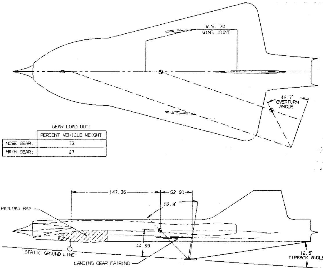
Figure 5.5: Conventional Landing Gear Layout
