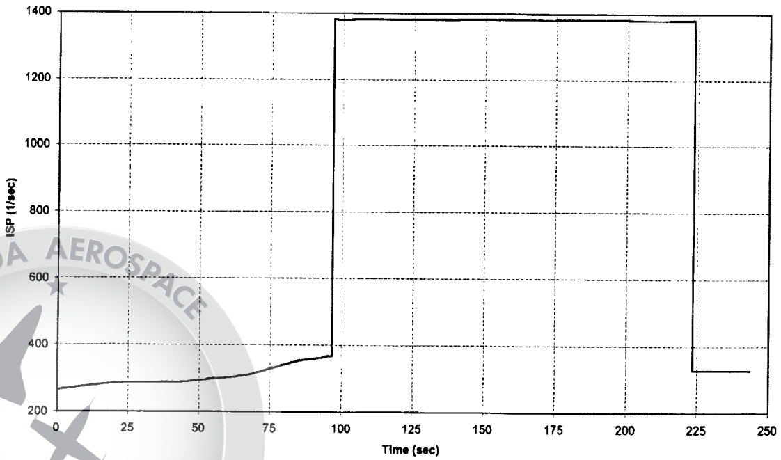
NASAE3CTLOX/ProB4 Specific Impulse vs Time
