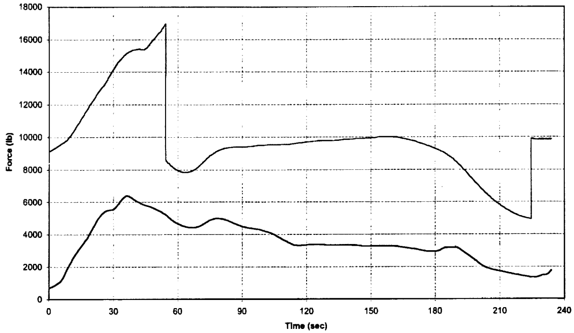
NASAE3GTLOX/PRA Thrust & Drag vs Time
