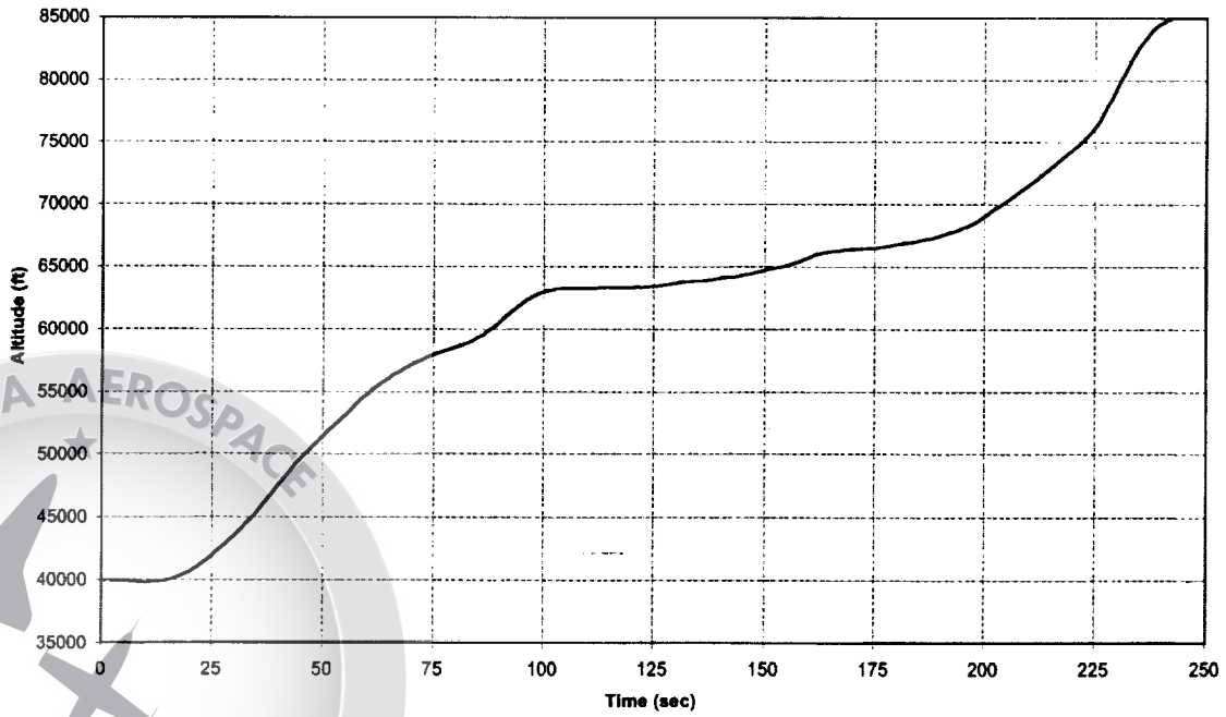
NASAE3CTLOX/ProB4 Altitude vs Time
