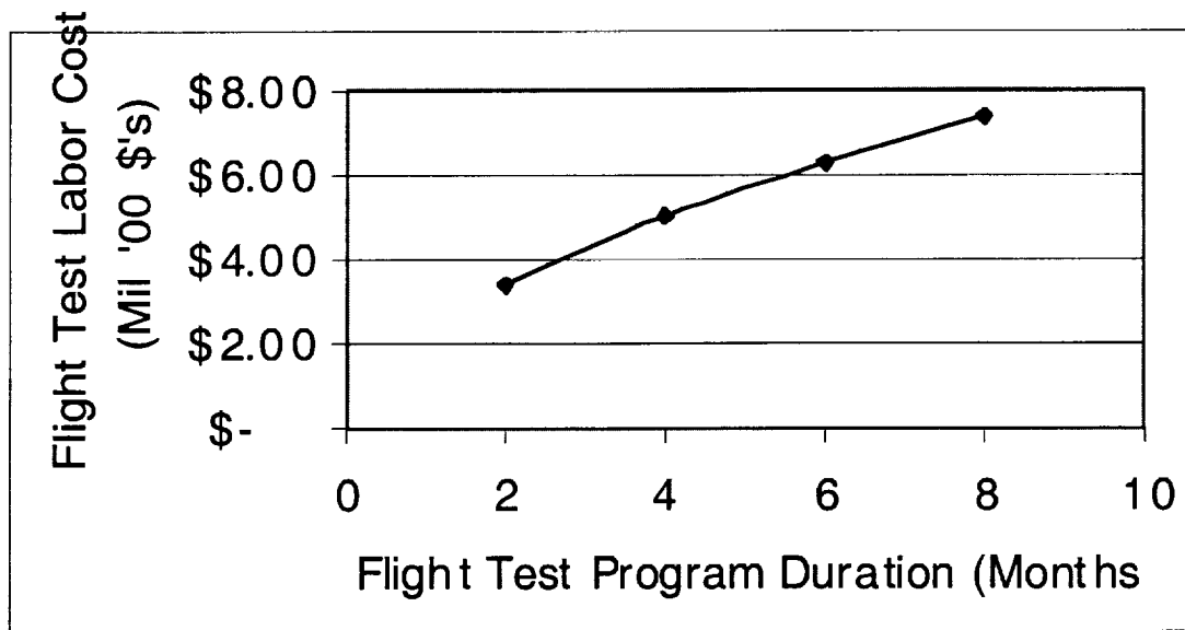
Figure 9.4. Flight Test Cost as a Function of Flight Test Program Duration
