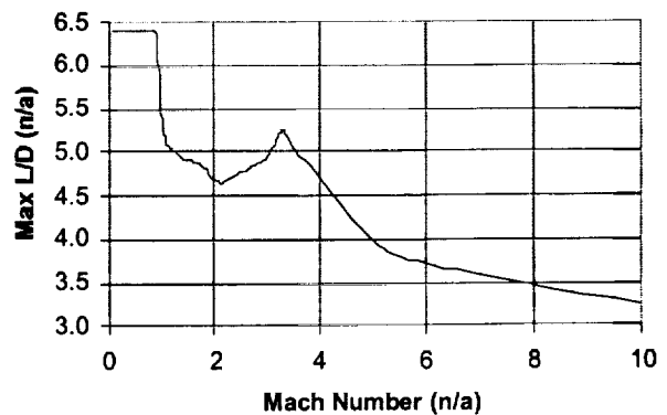
Figure 4.2: Maximum L/D vs Mach Number
