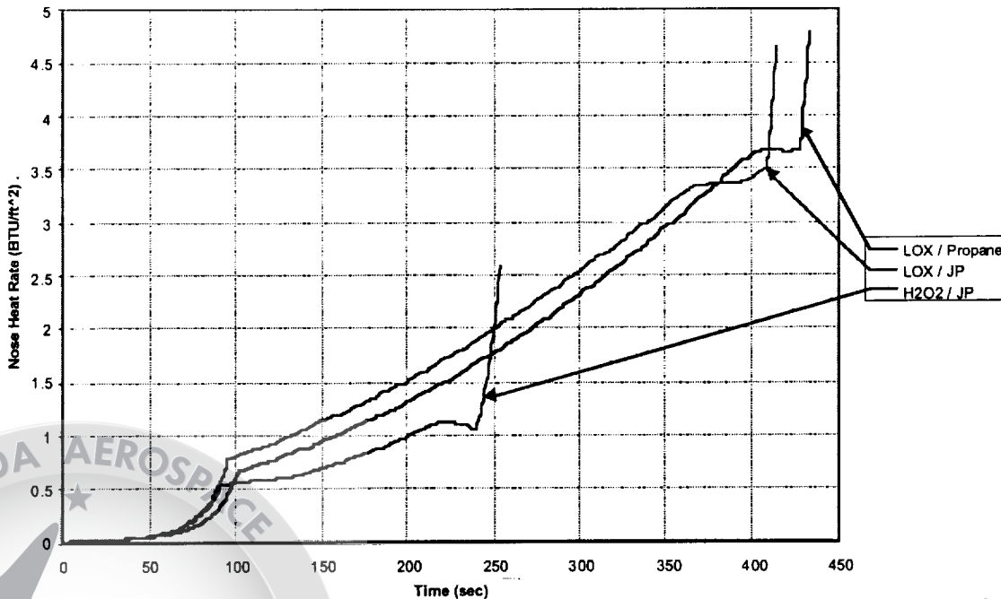
Figure 4.4: Final Trajectory Propellant Heat Rate Profiles
