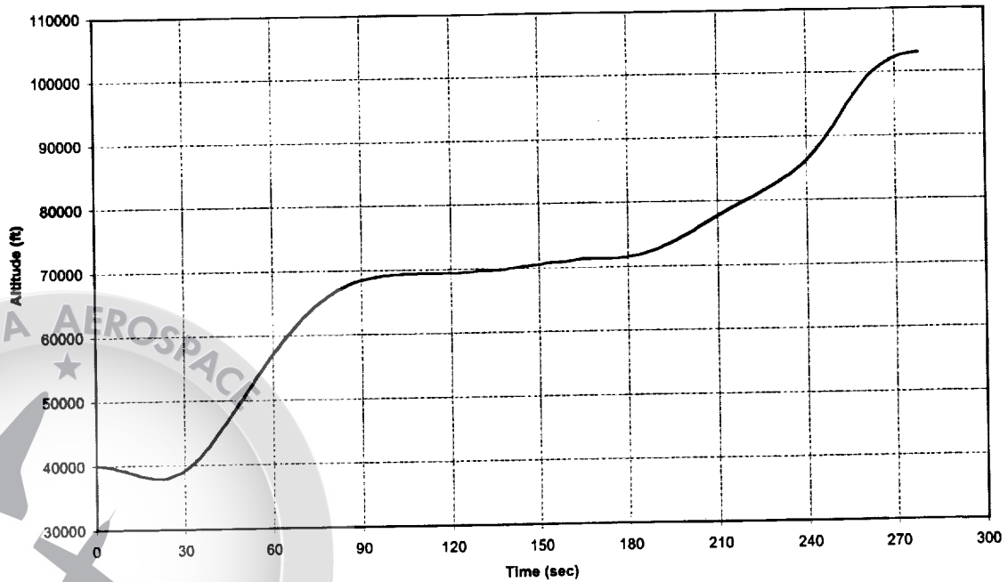
NASAE3GTH2O2/JPA Altitude vs Time
