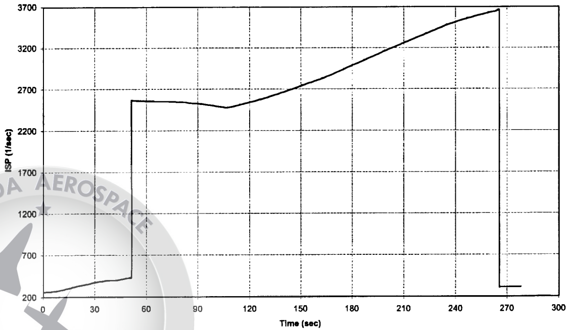
NASAE3GTH2O2/JPA Specific Impulse vs Time
