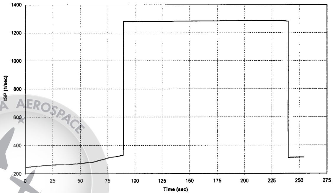
NASAE3CTH2O2/JPC1 Specific impulse vs Time
