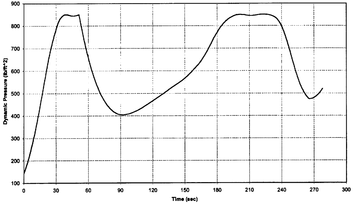
NASAE3GTH2O2/JPA Dynamic Pressure vs Time
