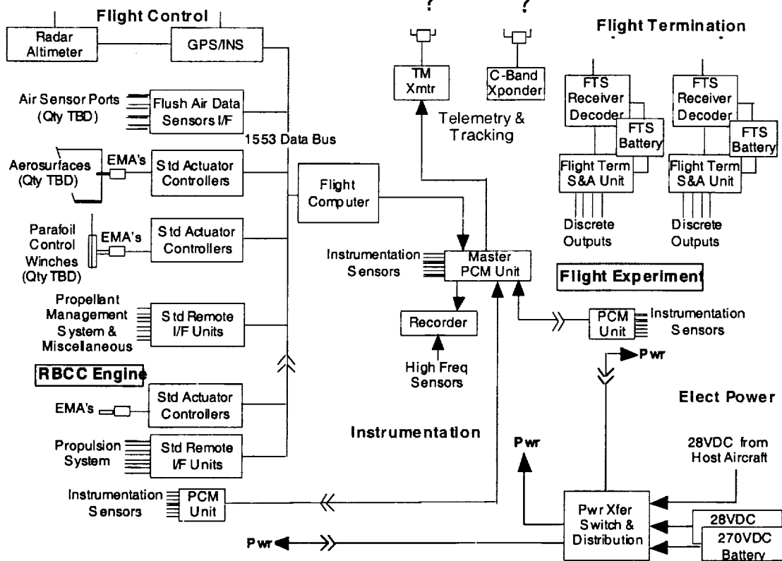
Figure 5.6: Conceptual Avionics Architecture
