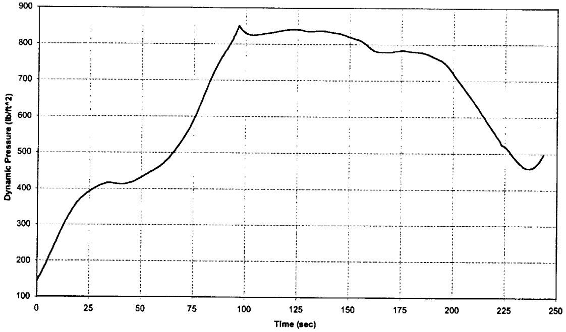
NASAE3CTLOX/ProB4 Dynamic Pressure vs Time
