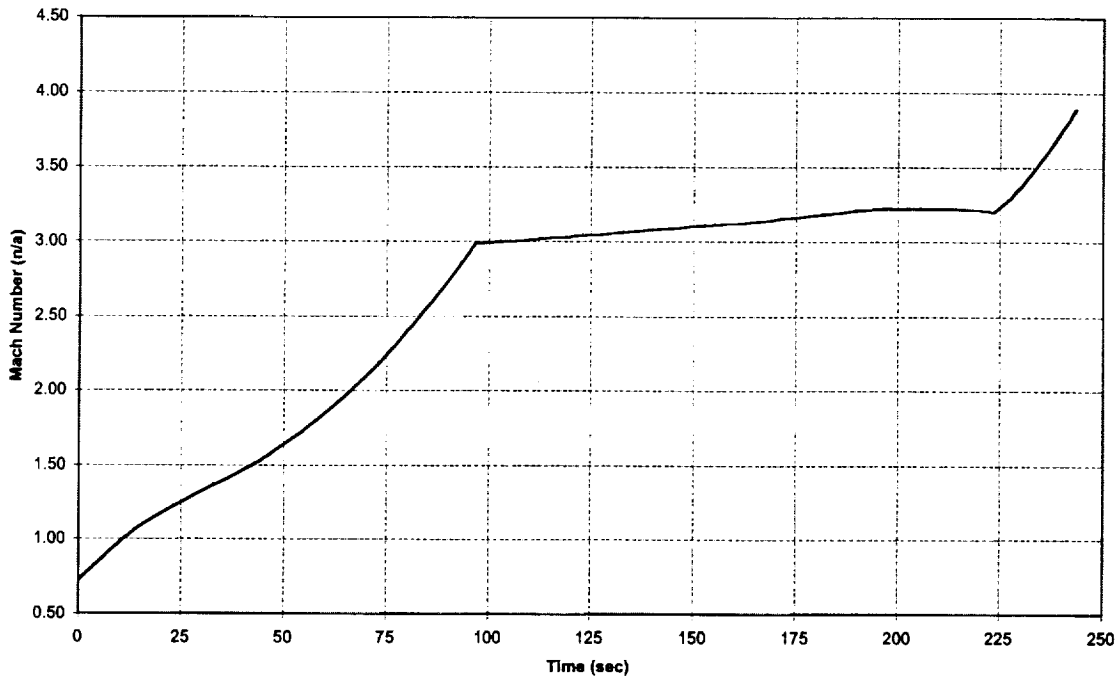
NASAE3CTLOX/ProB4 Mach vs Time
