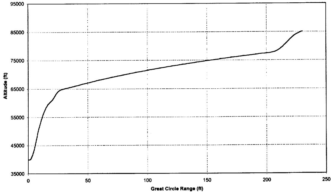
NASAE3CTLOX/ProC1 Altitude vs Great Circle Range
