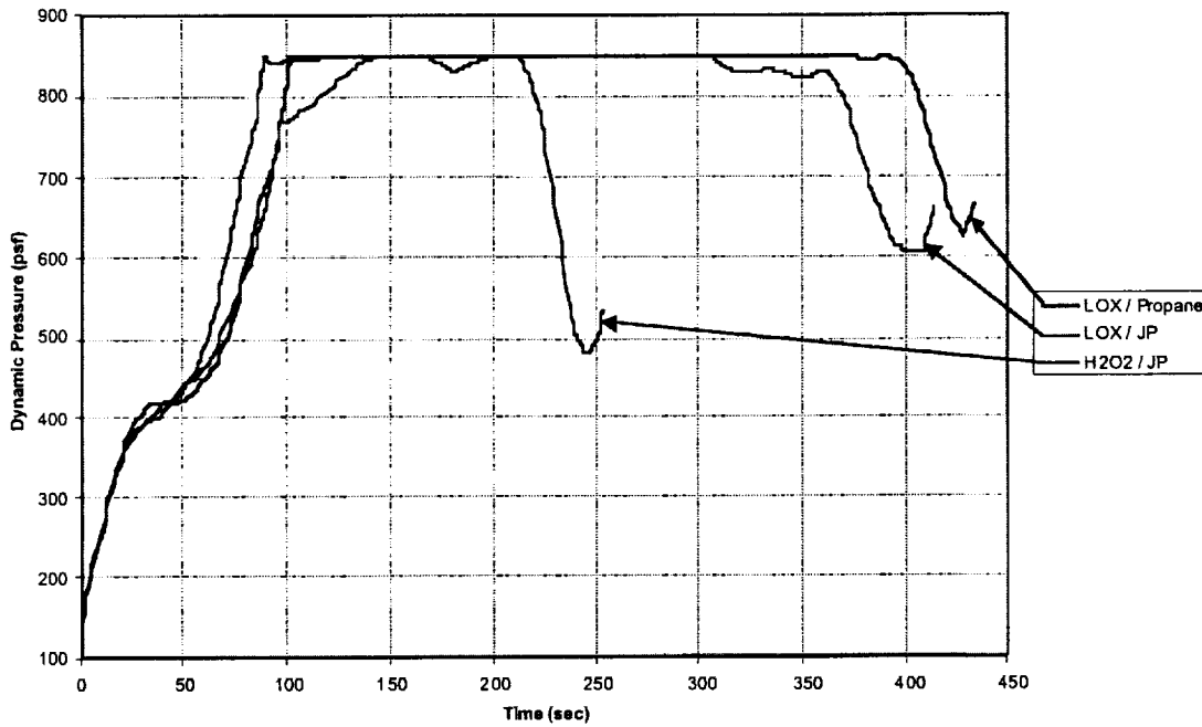
Figure 4.3: Final Trajectory Propellant Dynamic Pressure Profiles
