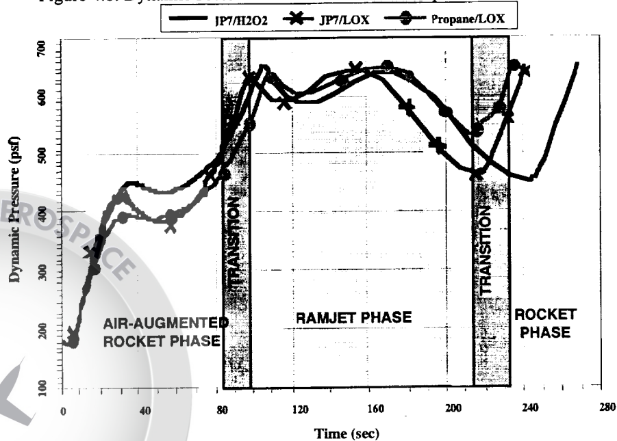
Figure 4.8: Dynamic Pressure Profile for Various Propellant Combinations
