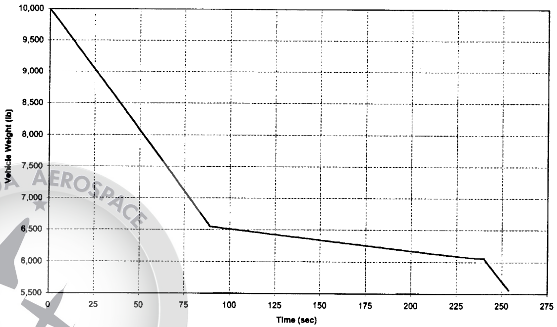
NASAE3CTH2O2/JPC1 Weight vs Time
