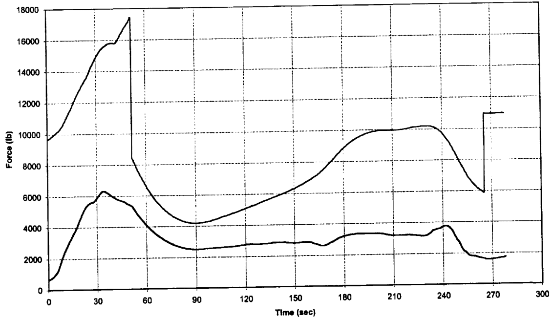
NASAE3GTH2O2/JPA Thrust & Drag vs Time
