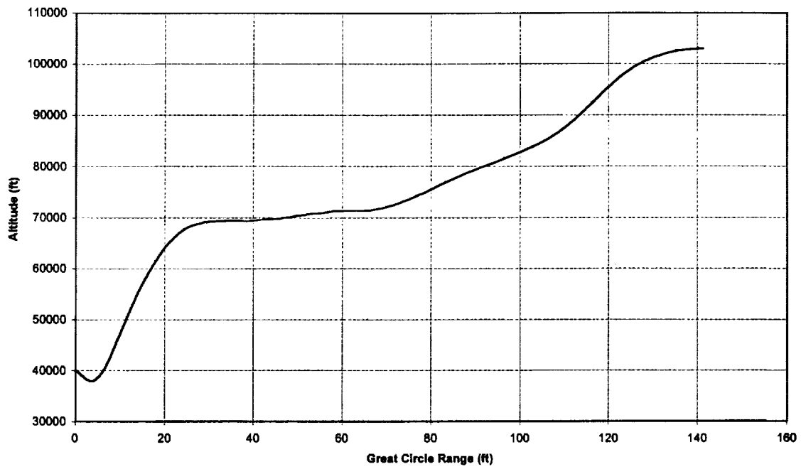
NASAE3GTH2O2/JPA Altitude vs Great Circle Range
