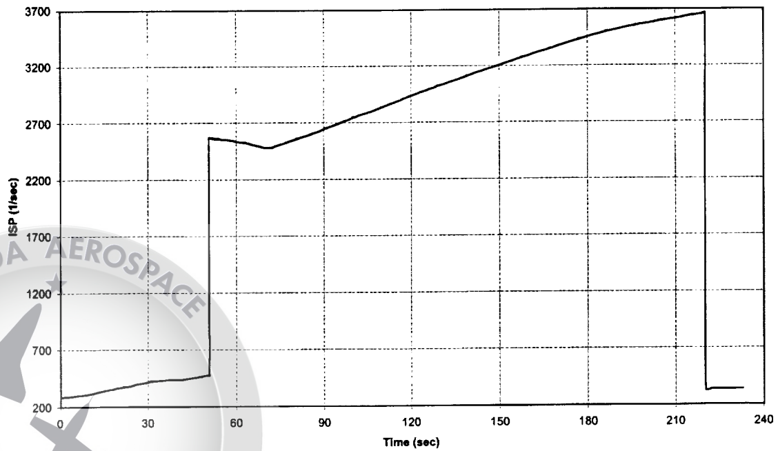
NASAE3GTLOX/JPA Specific Impulse vs Time
