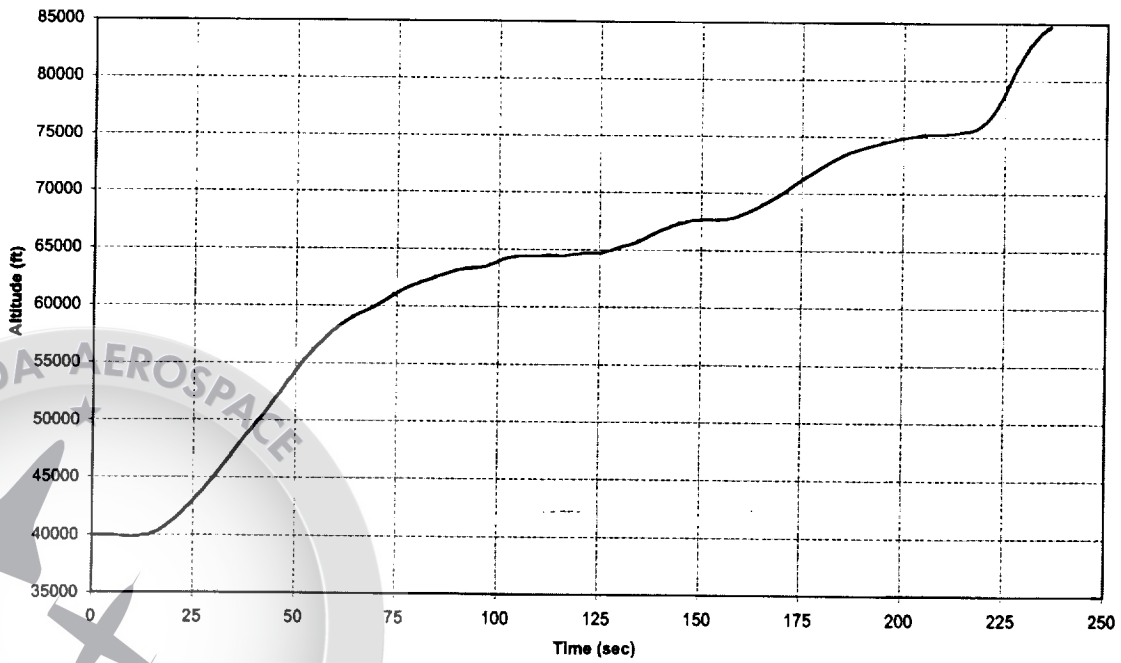
NASAE3CTLOX/JPB4 Altitude vs Time
